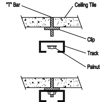
Drop Ceiling
