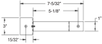
EBK - End Mounting Bracket
