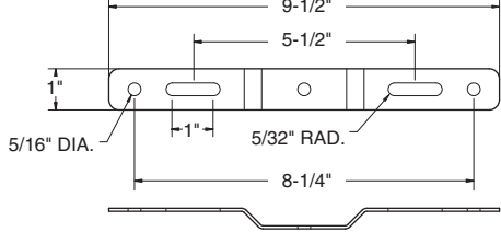
TBK - Top Mounting Bracket
