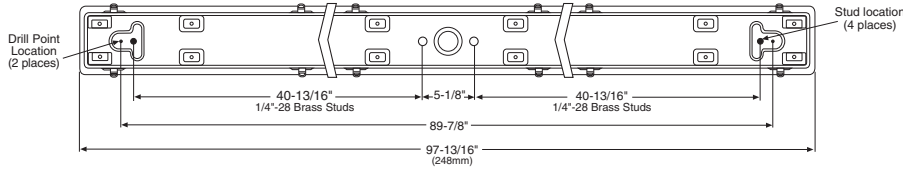
TBK - Top Mounting Bracket
