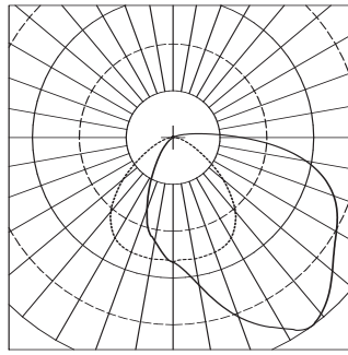
BIS175MXX-NAT-D10 90:..... 0: — TEST NUMBER: 26261 LAMP: 175W MH, COATED LUMENS: 15,000 MOUNTING HEIGHT: 12 FEET
