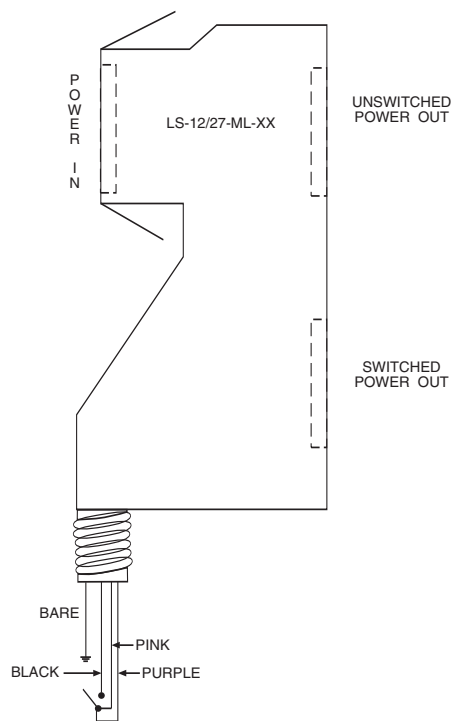
MULTI-LEVEL UNIT WIRED FOR SINGLE-LEVEL CONTROL
