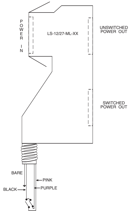
MULTI-LEVEL UNIT WIRED FOR SINGLE-LEVEL CONTROL
