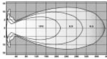
Vertical Distribution Feet From Lamp (Measured on Axis)
