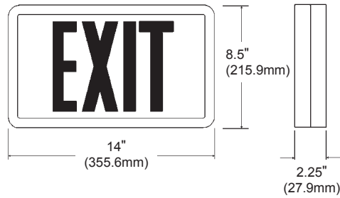
Plastic Frame - Double Face
