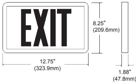
Aluminum Frame - Single Face
